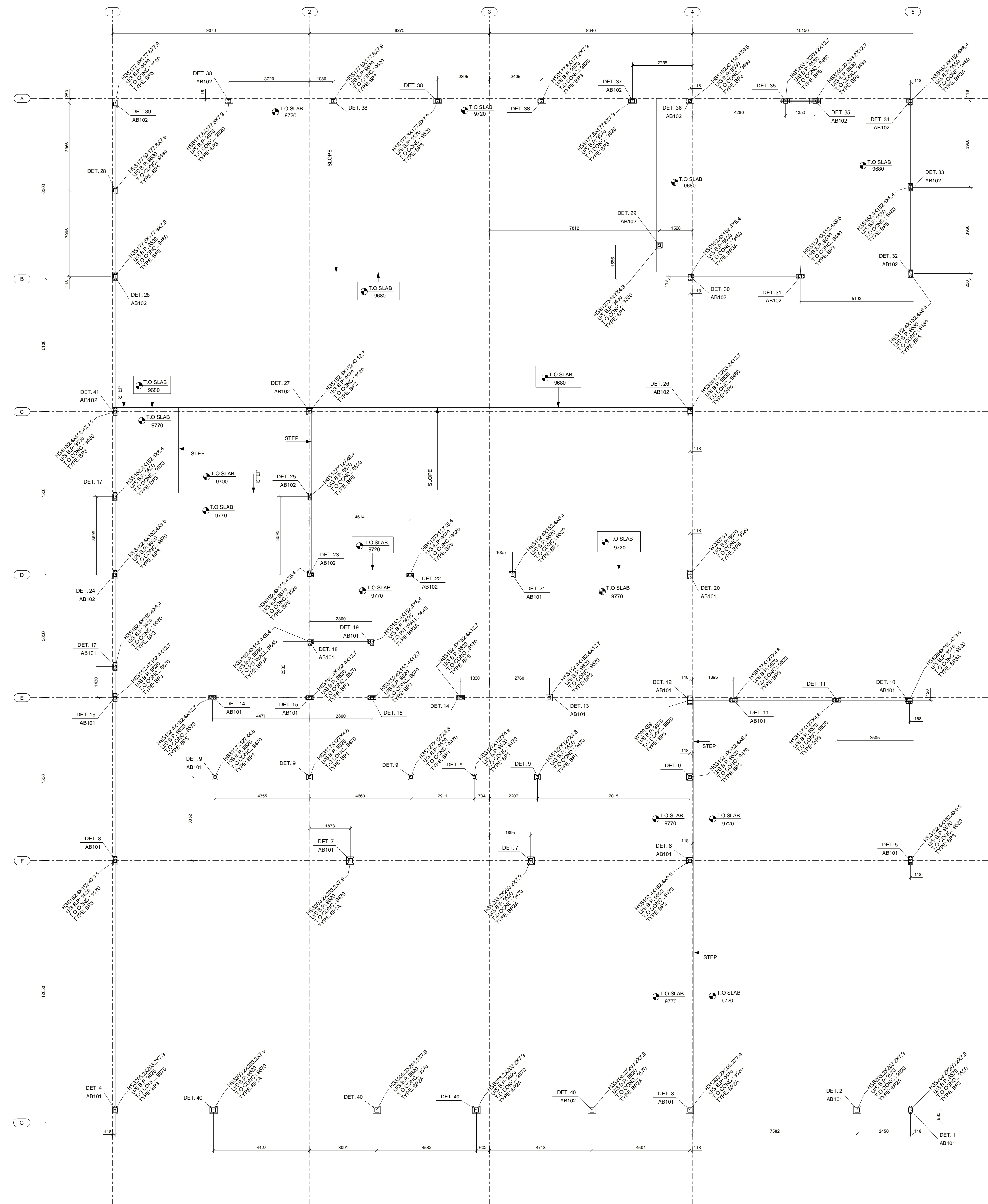
ANCHOR BOLT PLAN - MAIN FLOOR (EL. +9770)
